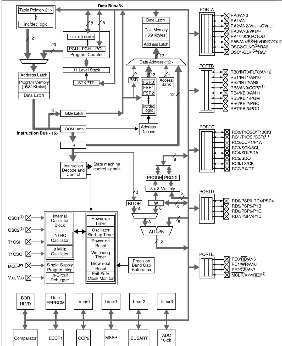
FIGURE 1-2: PIC18F4420/4520 (40/44-PIN) BLOCK DIAGRAM
