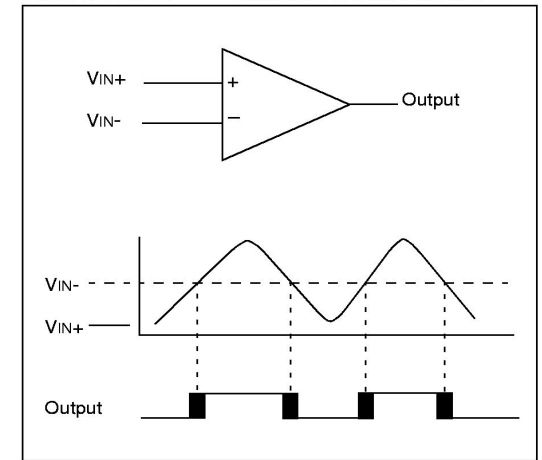
FIGURE 20-2: SINGLE COMPARATOR
