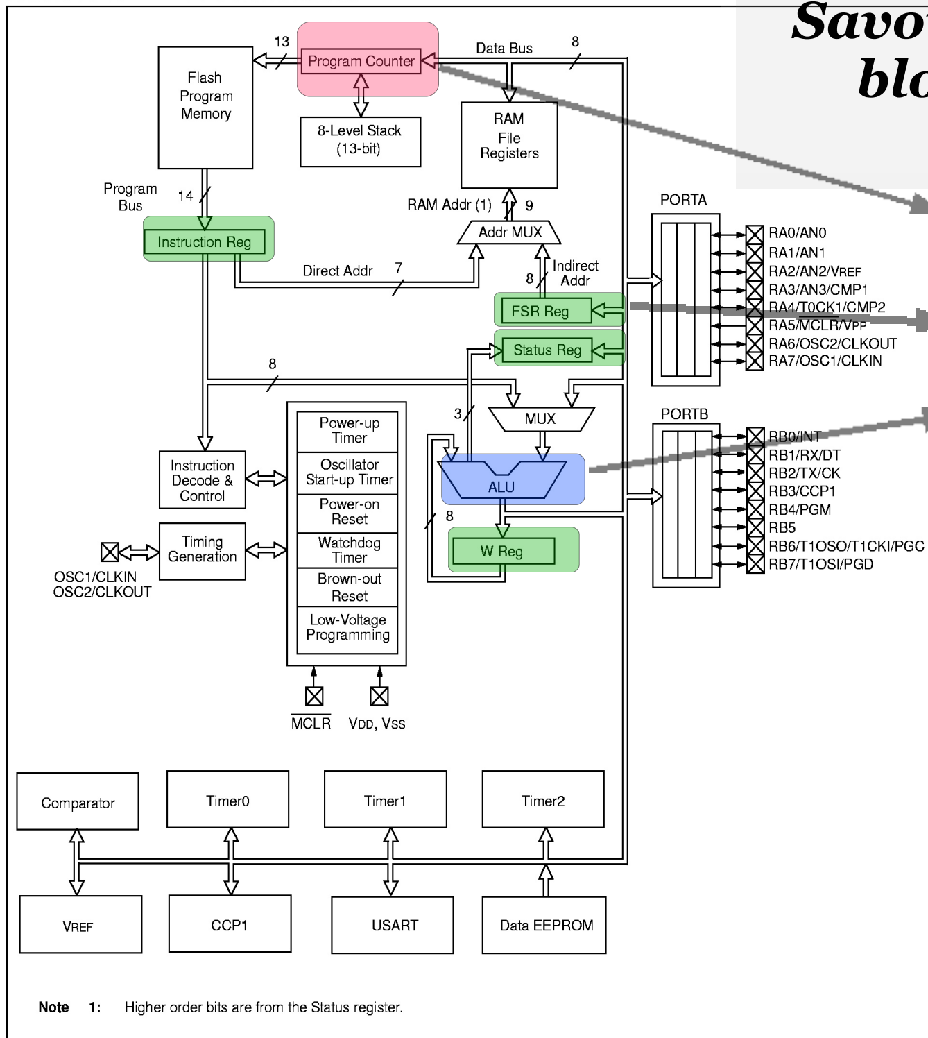
FIGURE 3-1: BLOCK DIAGRAM
