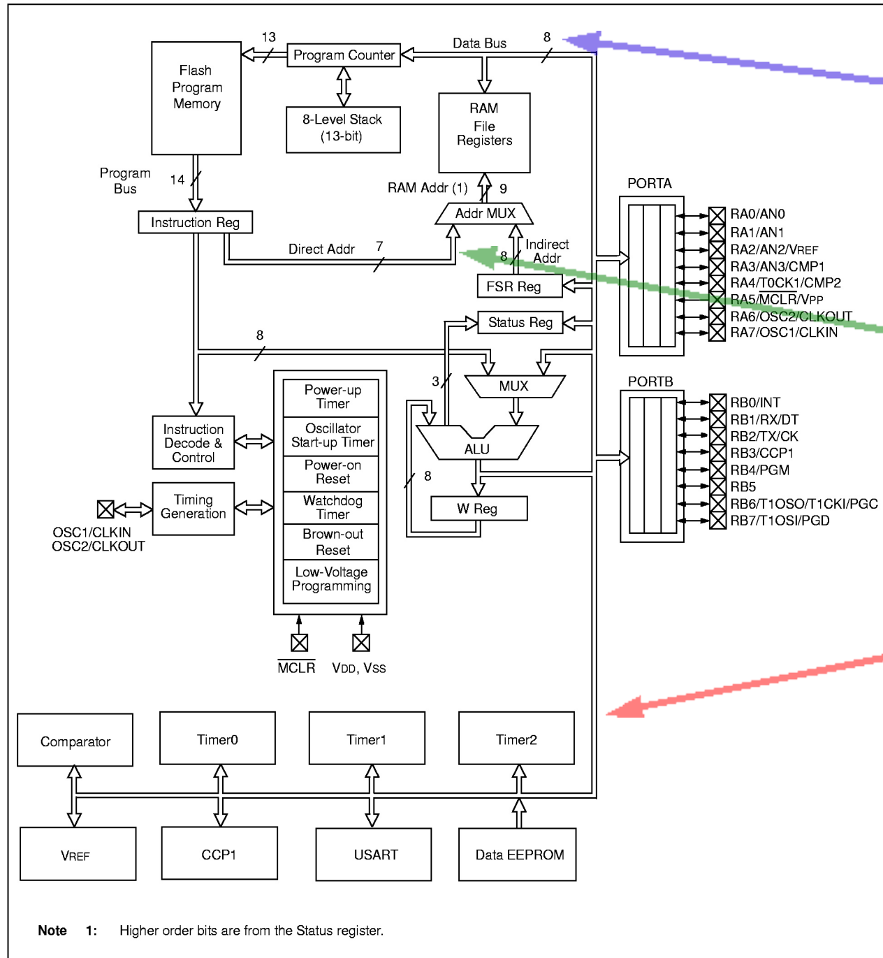
FIGURE 3-1: BLOCK DIAGRAM
