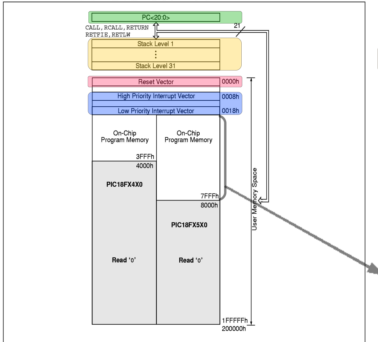
FIGURE 5-1: PROGRAM MEMORY MAP AND STACK FOR PIC18F2420/2520/4420/4520 DEVICES
