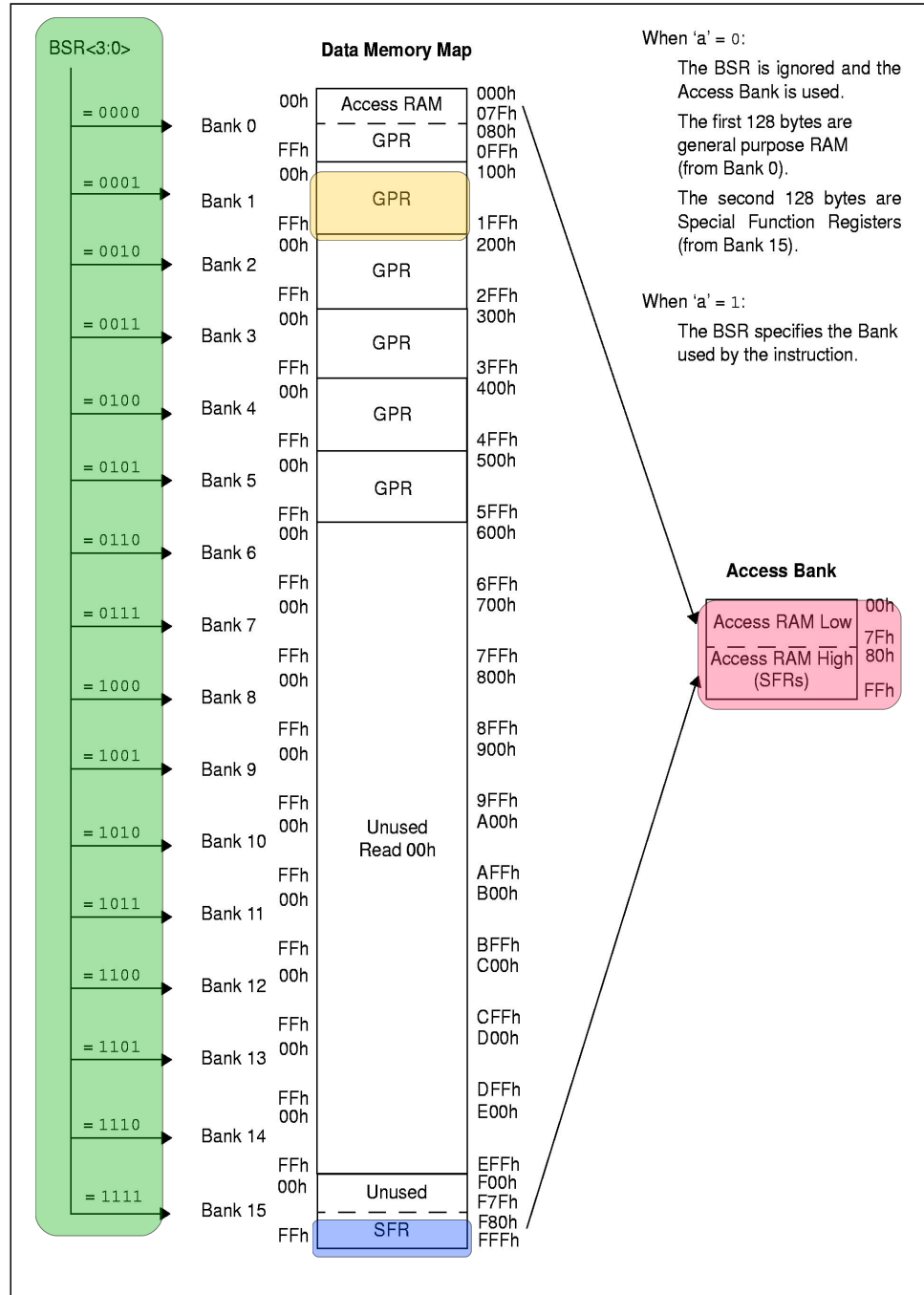
FIGURE 5-6: DATA MEMORY MAP FOR PIC18F2520/4520 DEVICES
