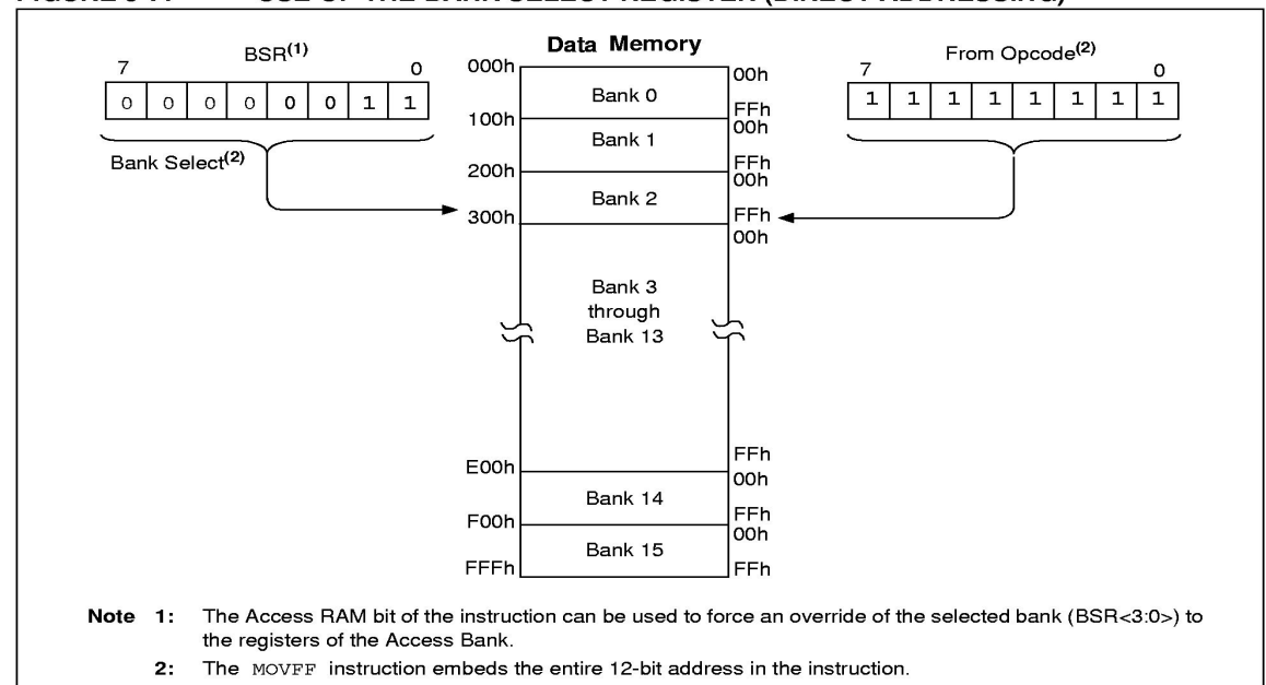
FIGURE 5-7: USE OF THE BANK SELECT REGISTER (DIRECT ADDRESSING)
