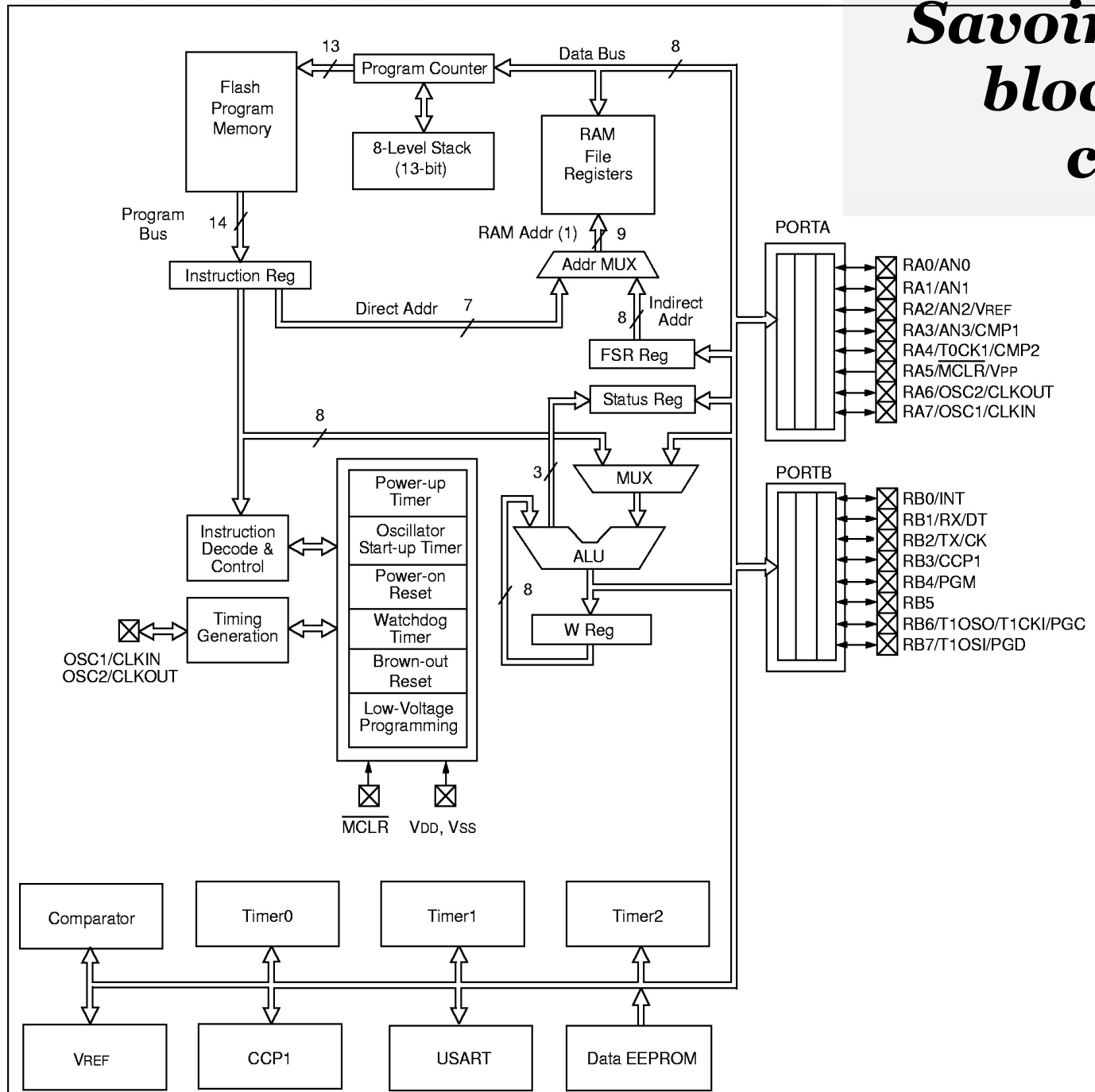
FIGURE 3-1: BLOCK DIAGRAM
