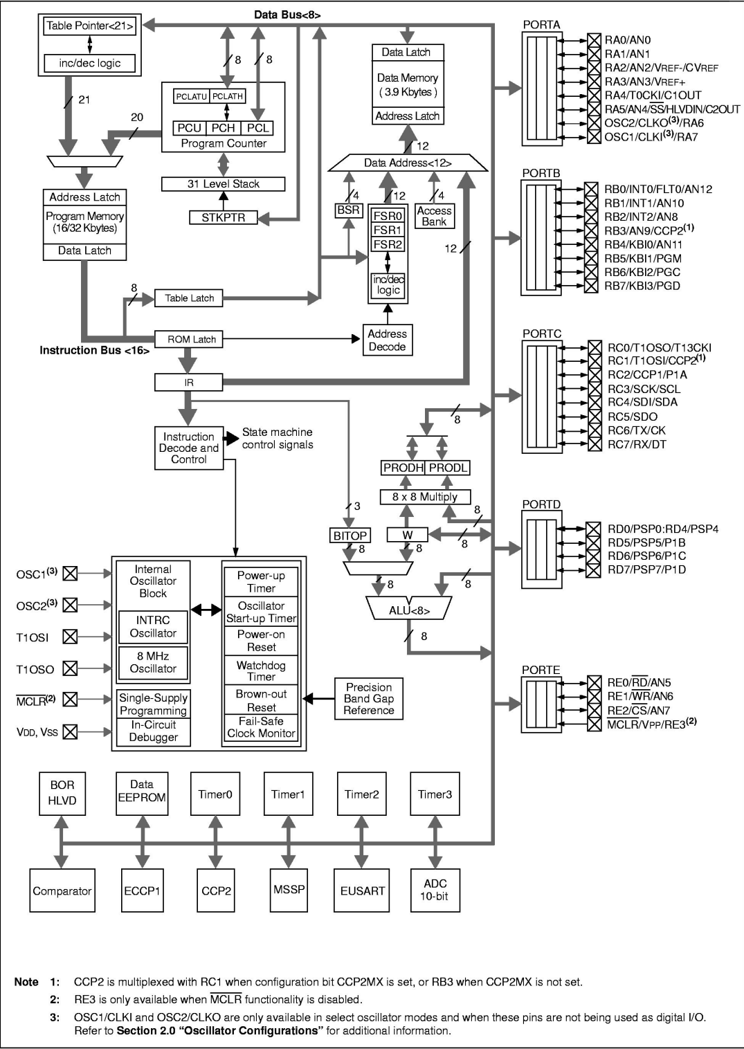
FIGURE 1-2: PIC18F4420/4520 (40/44-PIN) BLOCK DIAGRAM
