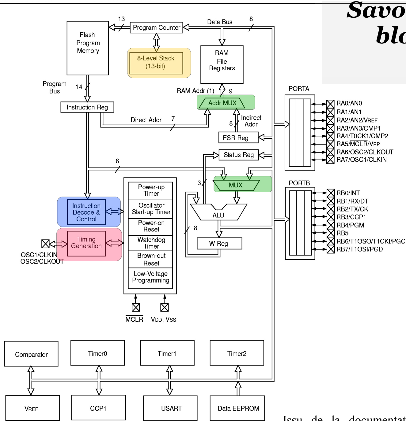
FIGURE 3-1: BLOCK DIAGRAM
