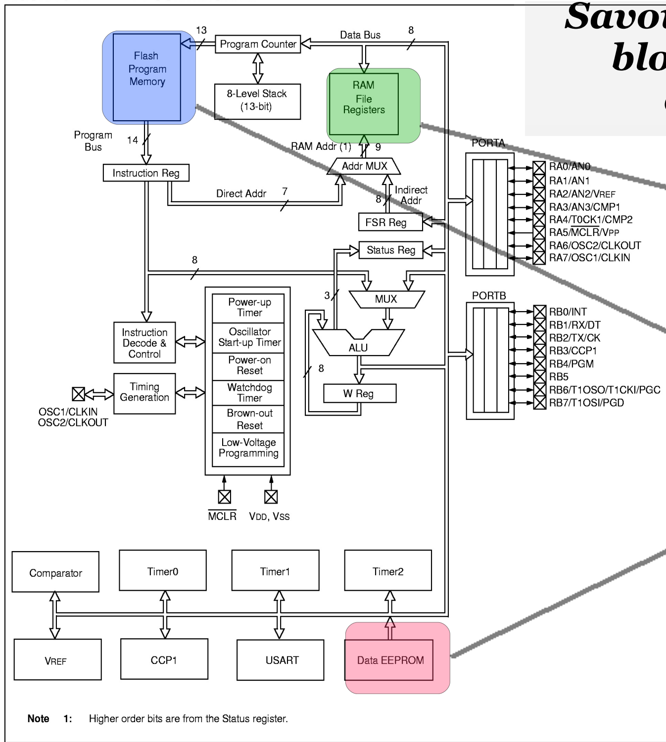
FIGURE 3-1: BLOCK DIAGRAM
