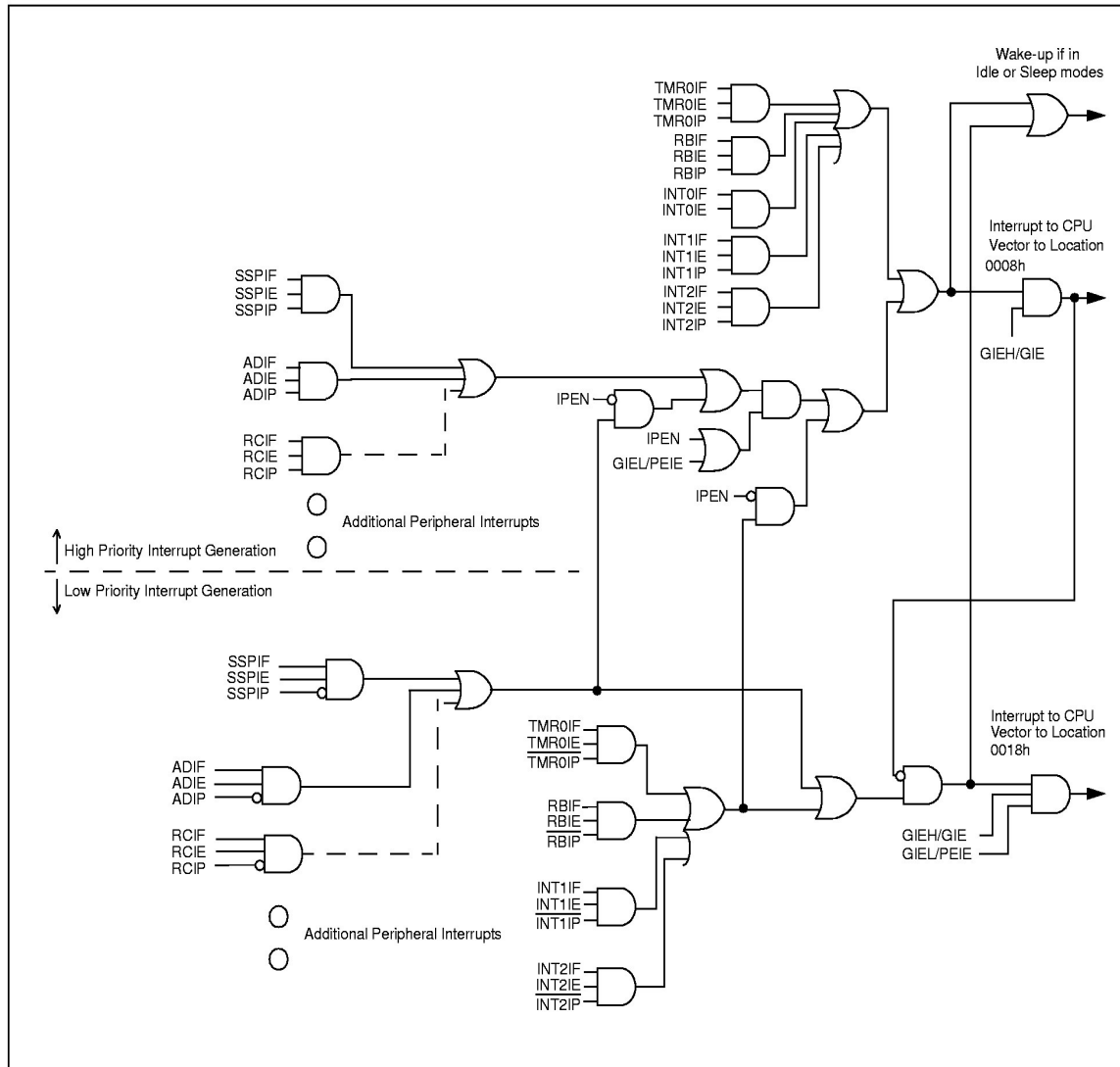
FIGURE 9-1: PIC18 INTERRUPT LOGIC
