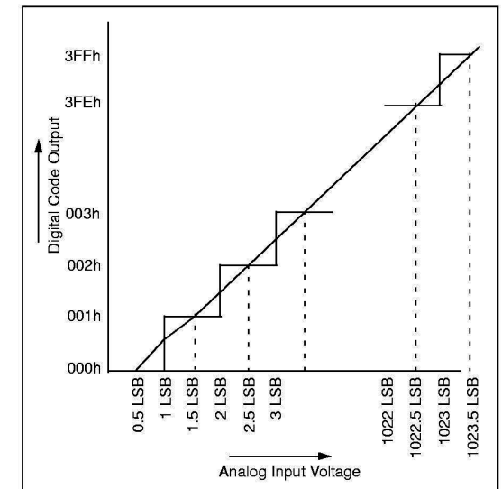
FIGURE 19-2: A/D TRANSFER FUNCTION
