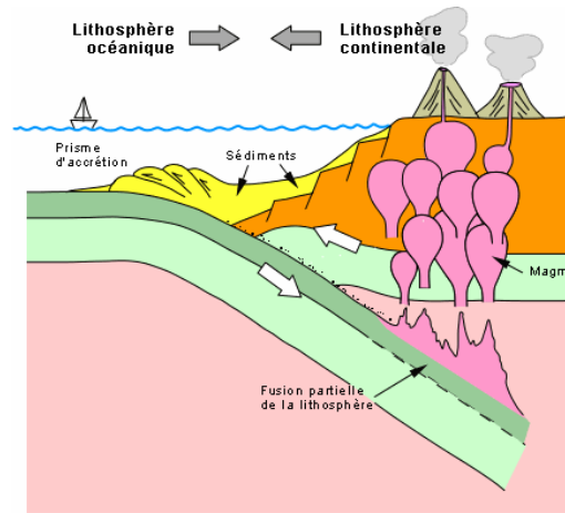
Figure.14. zone de subduction
